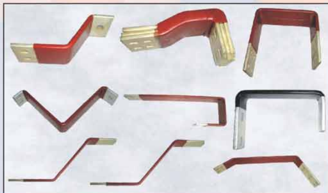
Raychem RPG's complete engineering solution for providing insulated busbars
